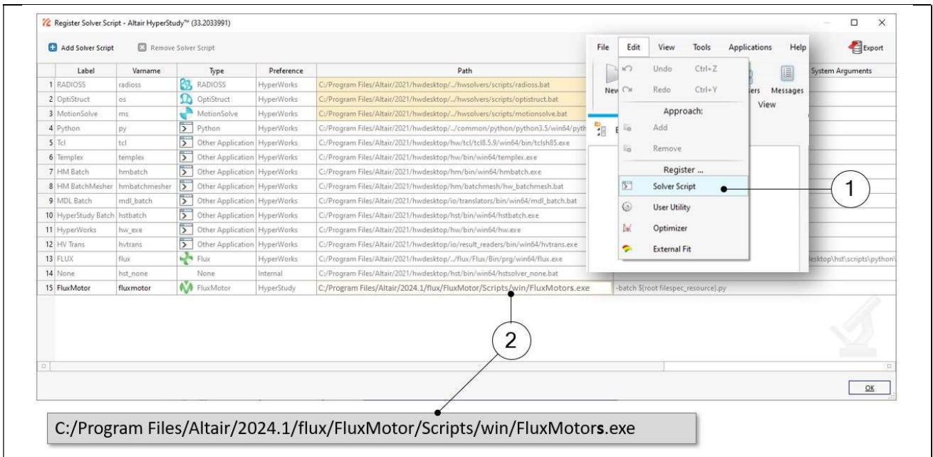
Connection between Altair FluxMotor™ and HyperStudy®
